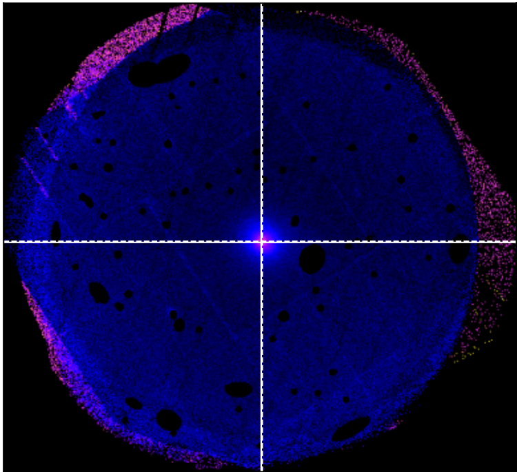
SDSSXCS-14 - Combined 0.5-2.0keV ratemap
