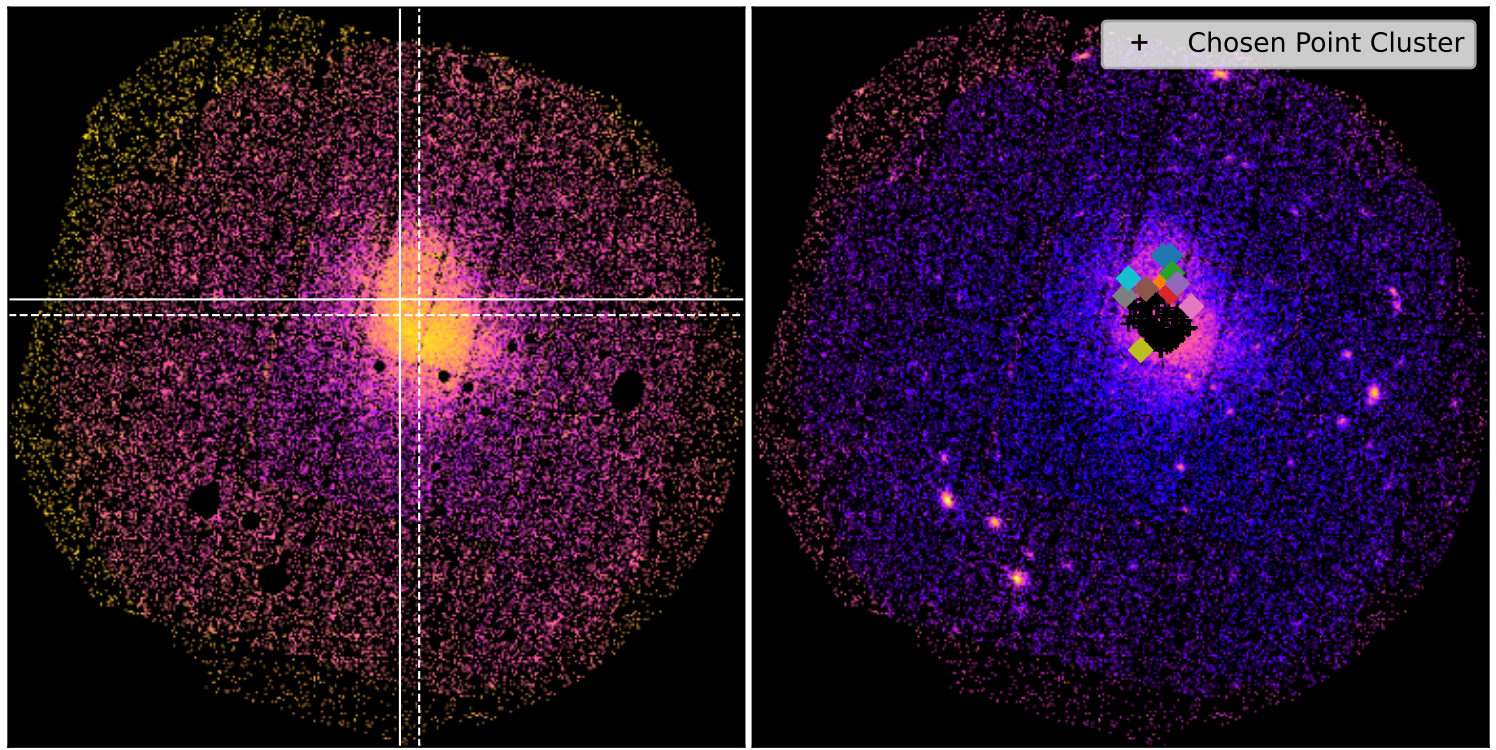
SDSSXCS-155 - Combined 0.5-2.0keV ratemapSDSSXCS-155 - Combined 0.5-2.0keV ratemap
