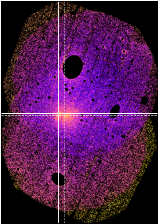
SDSSXCS-15 - Combined 0.5-2.0keV ratemap SDSSXCS-15 - Combined 0.5-2.0keV ratemap
