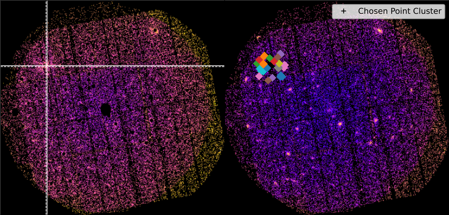
SDSSXCS-16286 - Combined 0.5-2.0keV ratemapSDSSXCS-16286 - Combined 0.5-2.0keV ratemap
