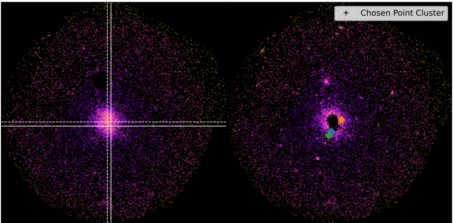
SDSSXCS-189 - Combined 0.5-2.0keV ratemapSDSSXCS-189 - Combined 0.5-2.0keV ratemap
