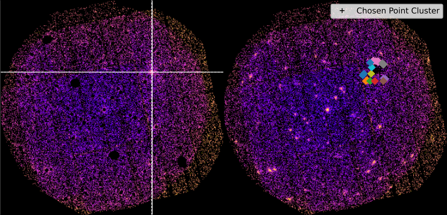
SDSSXCS-19922 - Combined 0.5-2.0keV ratemapSDSSXCS-19922 - Combined 0.5-2.0keV ratemap
