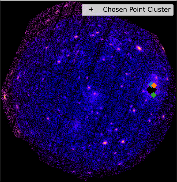
SDSSXCS-2092 - Combined 0.5-2.0keV ratemap
