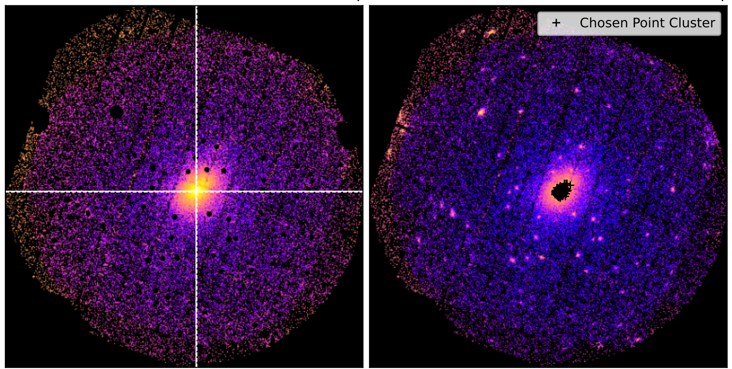
SDSSXCS-209 - Combined 0.5-2.0keV ratemapSDSSXCS-209 - Combined 0.5-2.0keV ratemap
