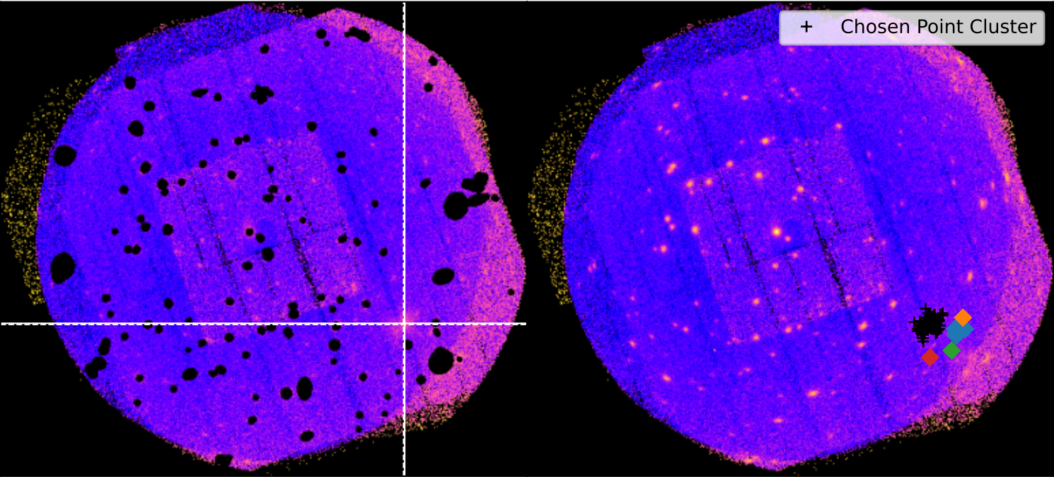
SDSSXCS-21847 - Combined 0.5-2.0keV ratemapSDSSXCS-21847 - Combined 0.5-2.0keV ratemap
