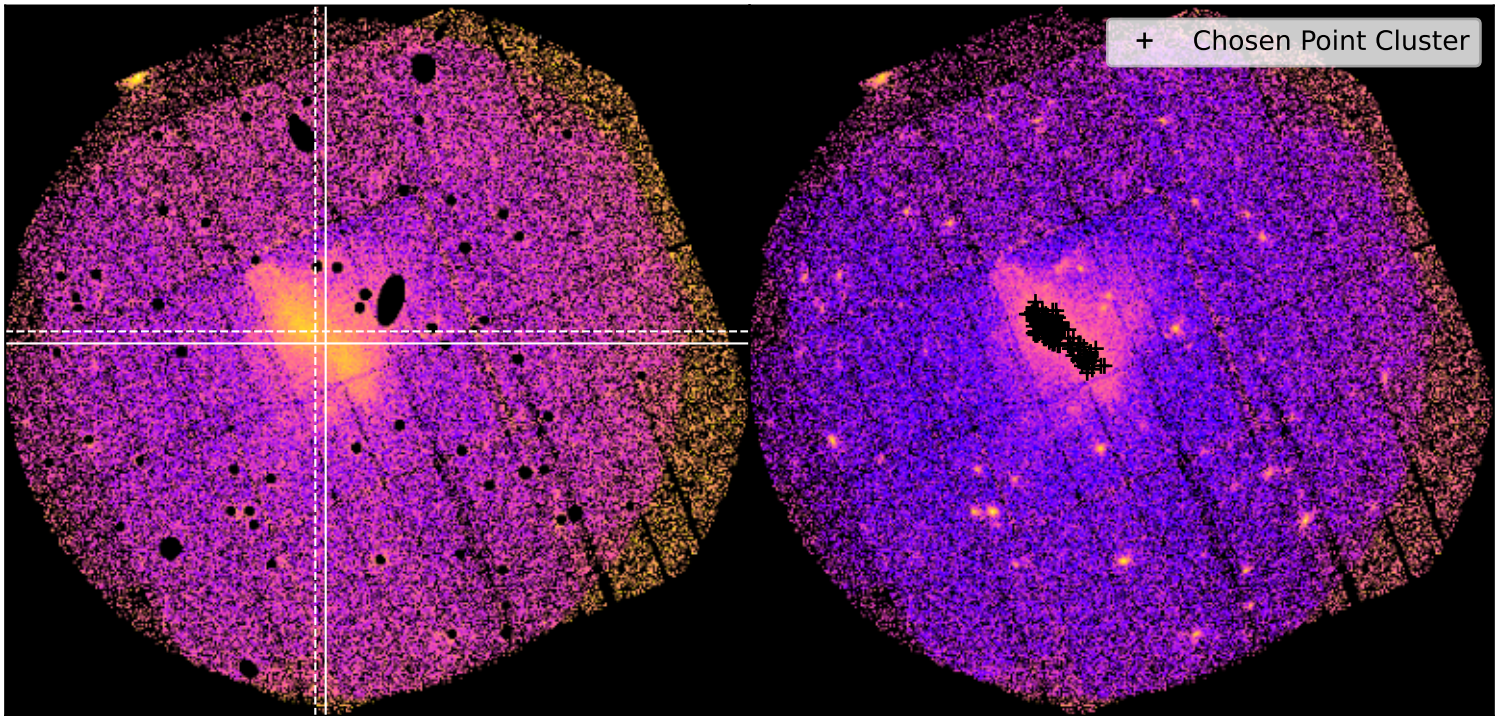
SDSSXCS-225 - Combined 0.5-2.0keV ratemapSDSSXCS-225 - Combined 0.5-2.0keV ratemap
