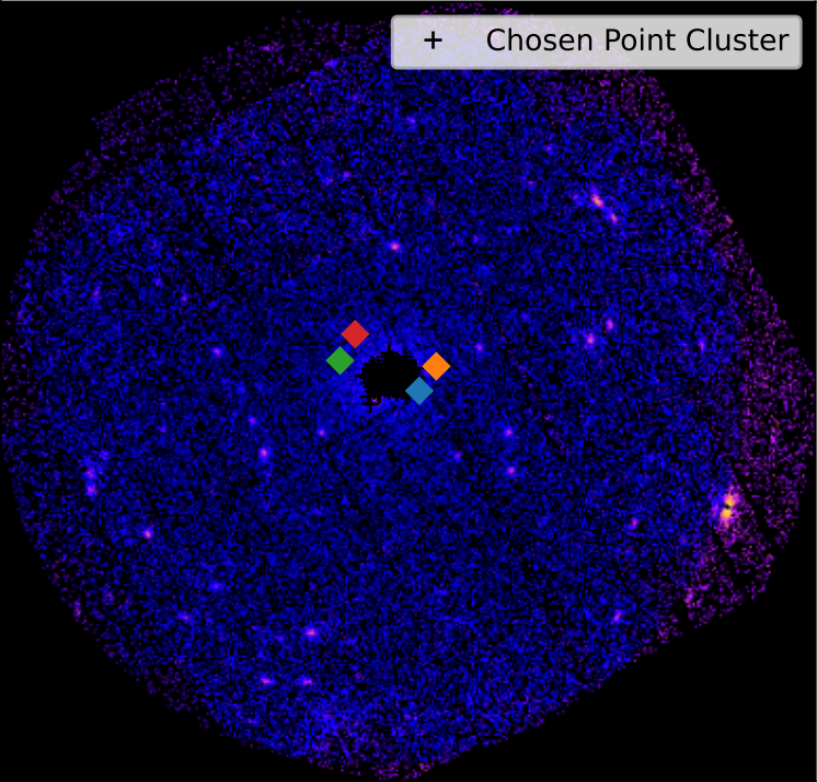
SDSSXCS-2347 - Combined 0.5-2.0keV ratemap
