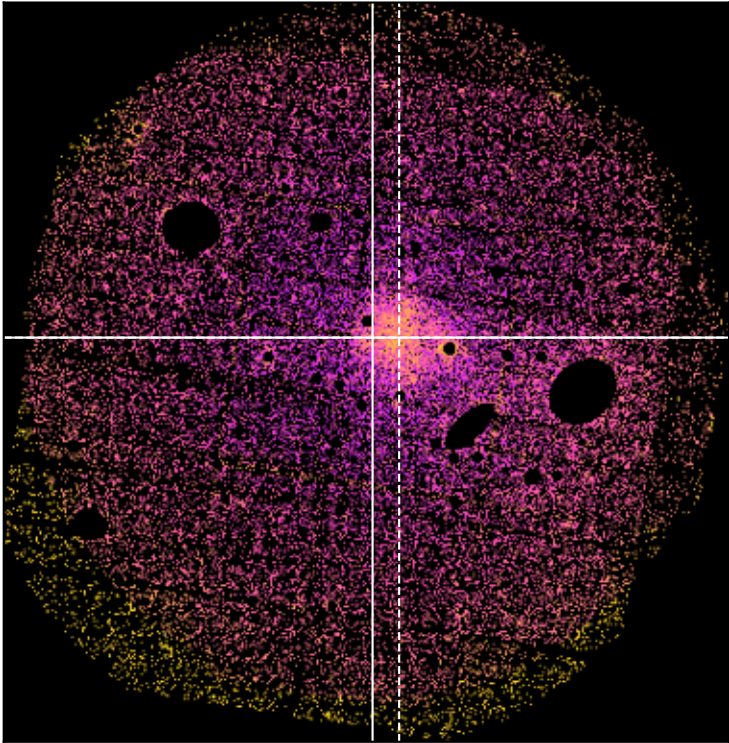
SDSSXCS-241 - Combined 0.5-2.0keV ratemapSDSSXCS-241 - Combined 0.5-2.0keV ratemap
