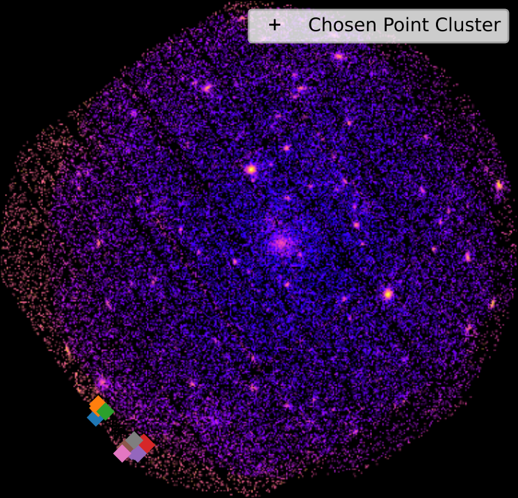
SDSSXCS-28269 - Combined 0.5-2.0keV ratemap
