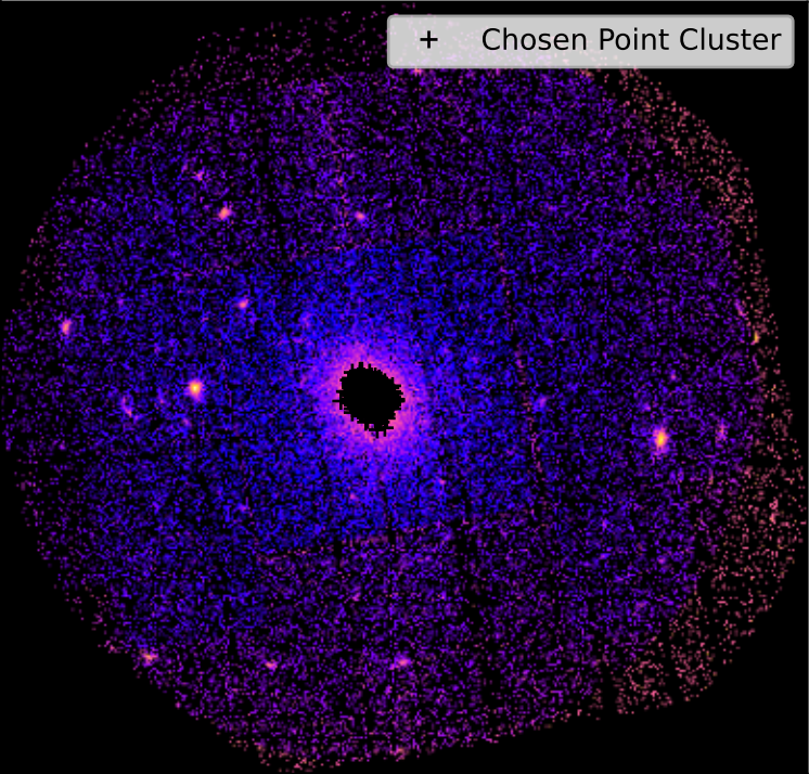
SDSSXCS-2836 - Combined 0.5-2.0keV ratemap
