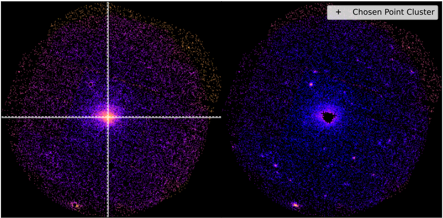
SDSSXCS-286 - Combined 0.5-2.0keV ratemapSDSSXCS-286 - Combined 0.5-2.0keV ratemap
