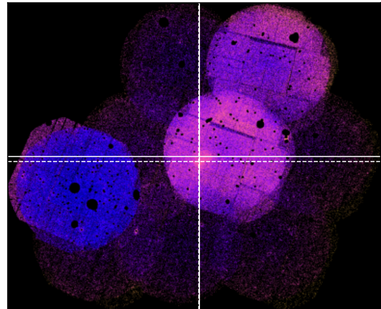
SDSSXCS-2984 - Combined 0.5-2.0keV ratemap
