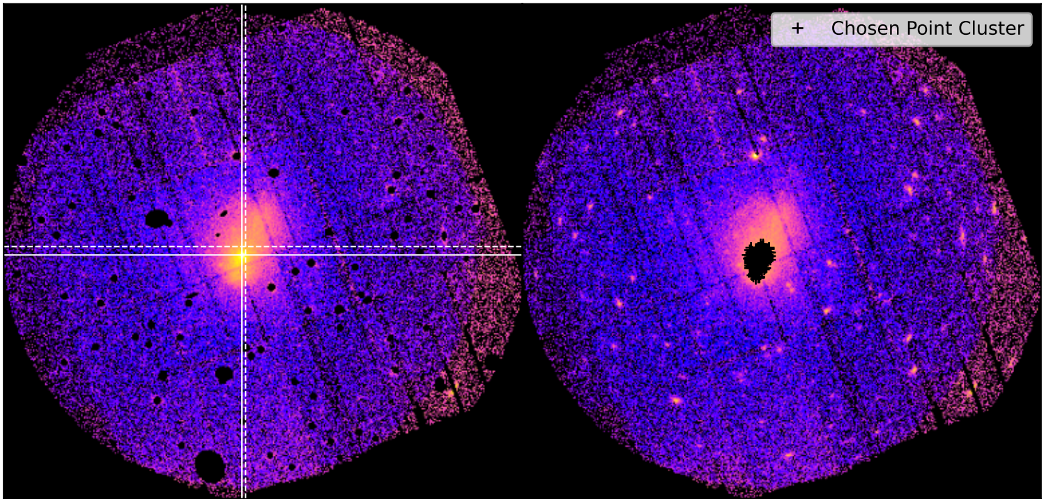
SDSSXCS-298 - Combined 0.5-2.0keV ratemapSDSSXCS-298 - Combined 0.5-2.0keV ratemap
