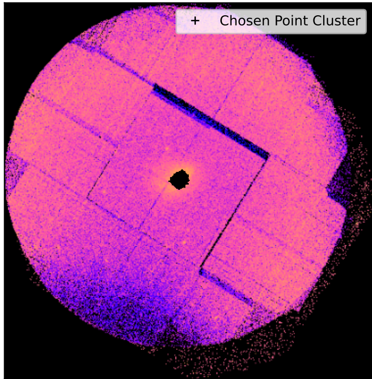
SDSSXCS-29 - Combined 0.5-2.0keV ratemap
