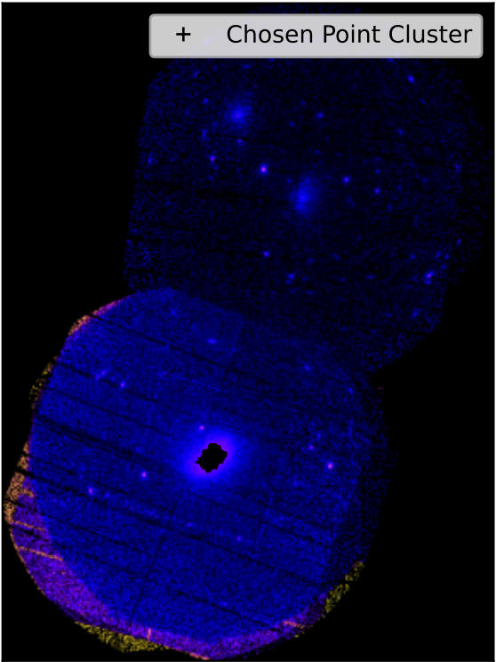
SDSSXCS-2 - Combined 0.5-2.0keV ratemap
