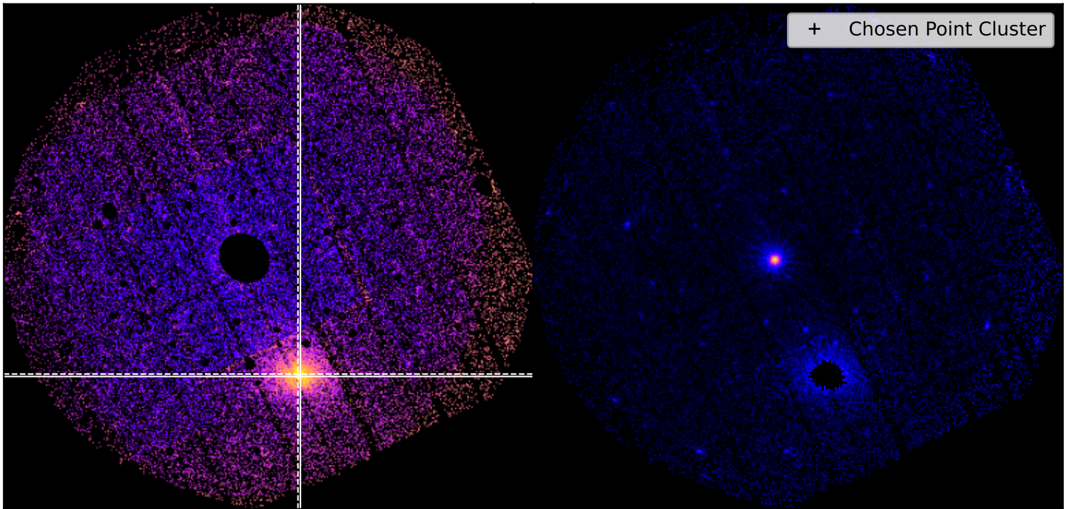
SDSSXCS-309 - Combined 0.5-2.0keV ratemapSDSSXCS-309 - Combined 0.5-2.0keV ratemap
