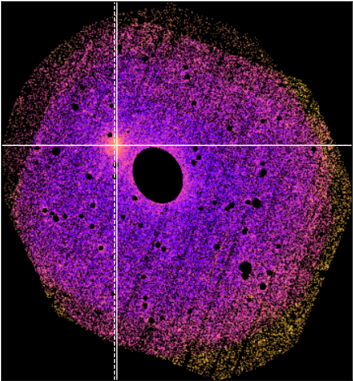
SDSSXCS-34 - Combined 0.5-2.0keV ratemap
