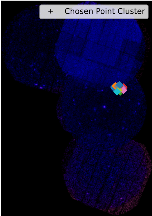
SDSSXCS-35404 - Combined 0.5-2.0keV ratemap
