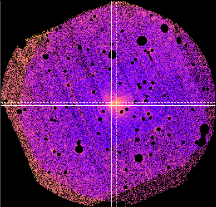
SDSSXCS-3746 - Combined 0.5-2.0keV ratemap
