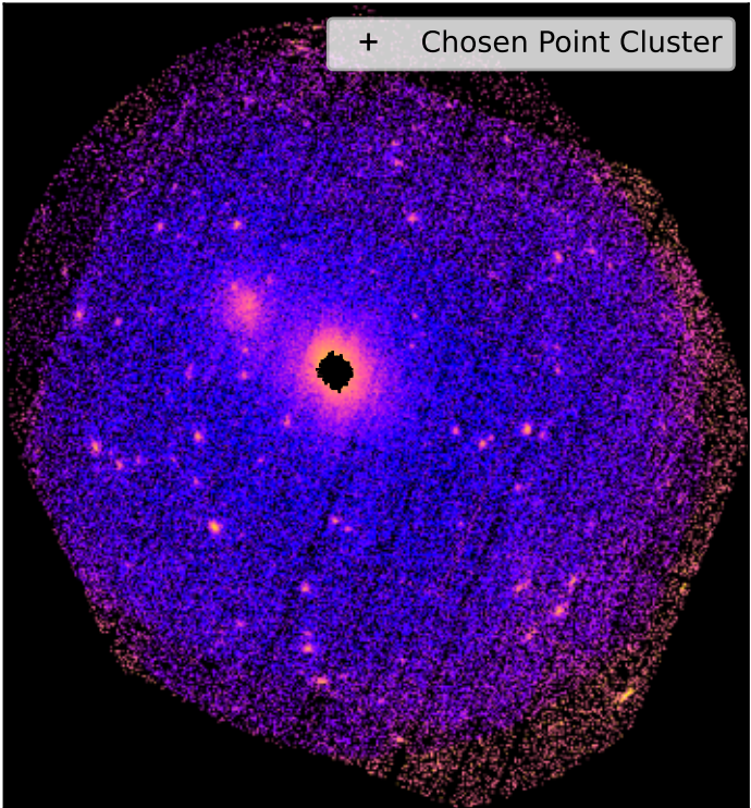
SDSSXCS-41 - Combined 0.5-2.0keV ratemap
