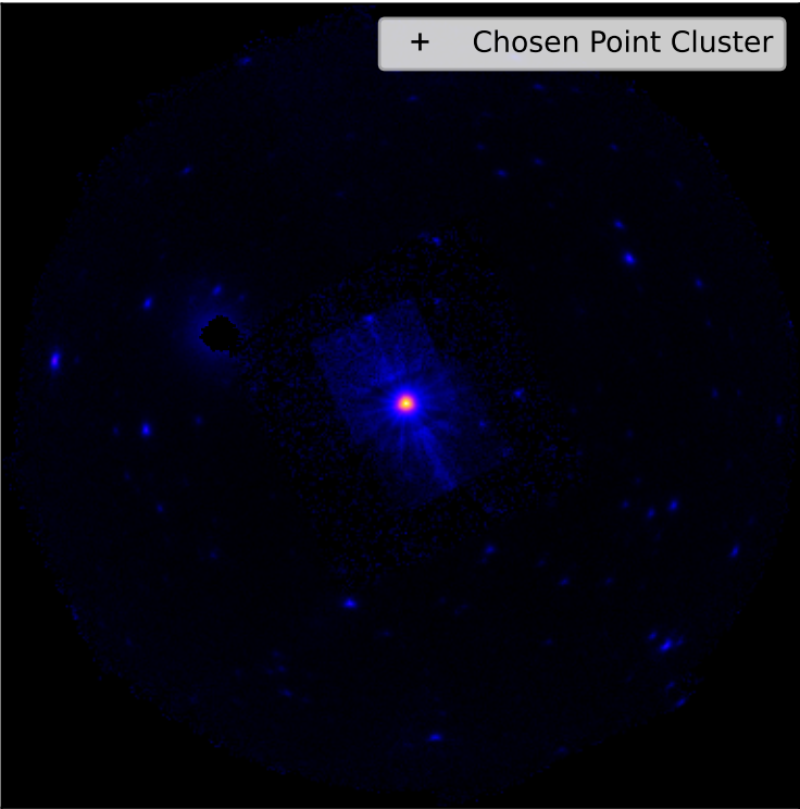
SDSSXCS-4313 - Combined 0.5-2.0keV ratemap
