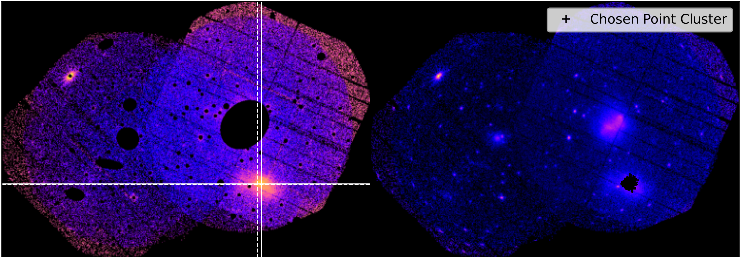
SDSSXCS-457 - Combined 0.5-2.0keV ratemapSDSSXCS-457 - Combined 0.5-2.0keV ratemap
