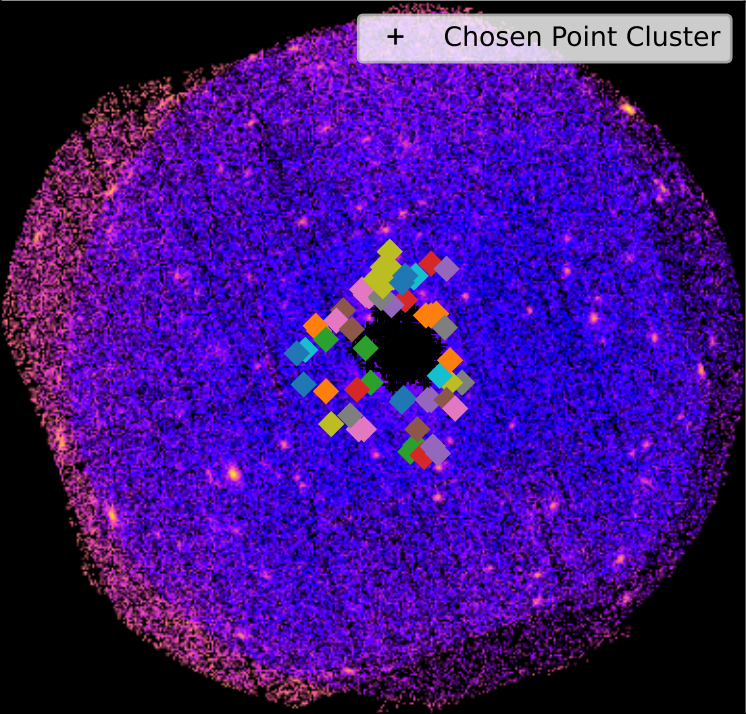
SDSSXCS-5159 - Combined 0.5-2.0keV ratemap
