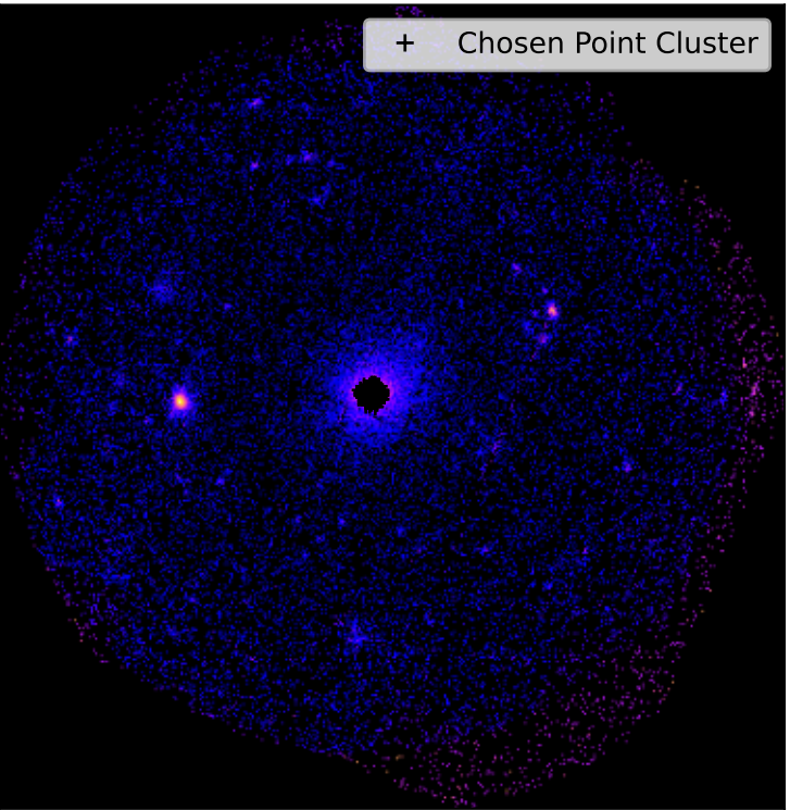
SDSSXCS-51 - Combined 0.5-2.0keV ratemap
