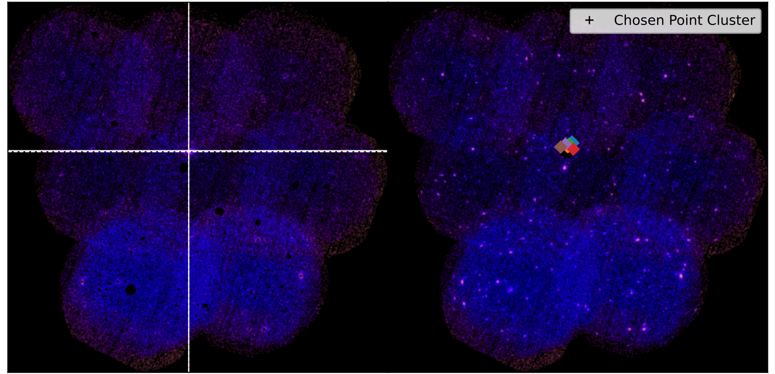
SDSSXCS-5743 - Combined 0.5-2.0keV ratemap
