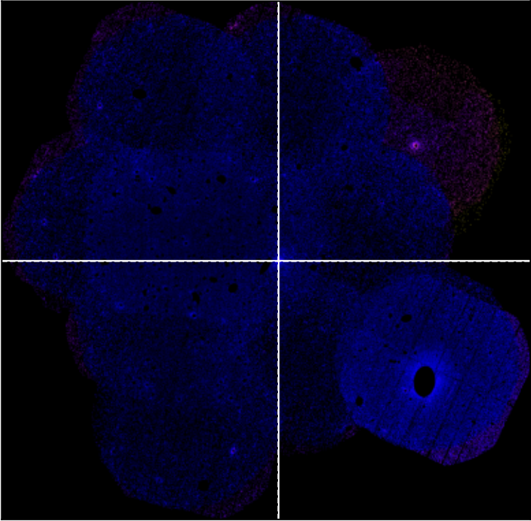
SDSSXCS-5830 - Combined 0.5-2.0keV ratemap
