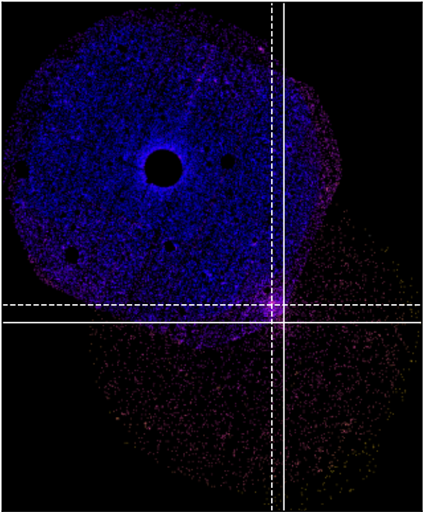
SDSSXCS-586 - Combined 0.5-2.0keV ratemapSDSSXCS-586 - Combined 0.5-2.0keV ratemap
