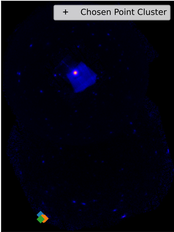
SDSSXCS-58896 - Combined 0.5-2.0keV ratemap
