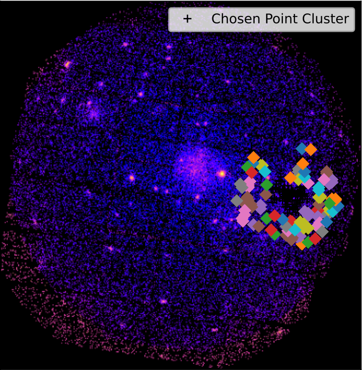
SDSSXCS-6307 - Combined 0.5-2.0keV ratemap
