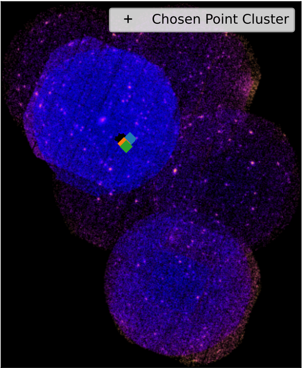
SDSSXCS-64824 - Combined 0.5-2.0keV ratemap
