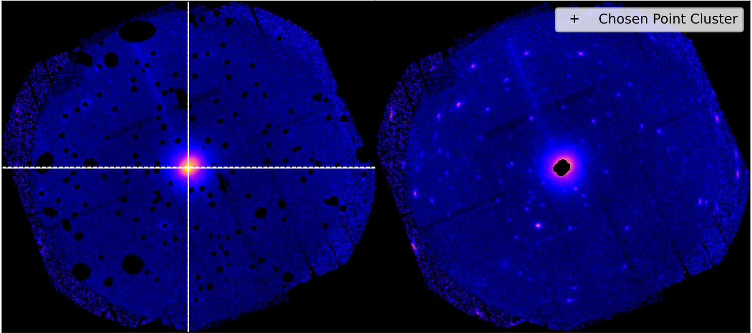
SDSSXCS-667 - Combined 0.5-2.0keV ratemapSDSSXCS-667 - Combined 0.5-2.0keV ratemap
