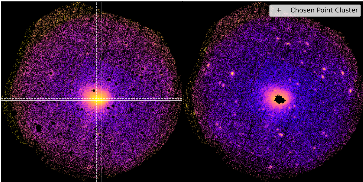
SDSSXCS-68 - Combined 0.5-2.0keV ratemap SDSSXCS-68 - Combined 0.5-2.0keV ratemap
