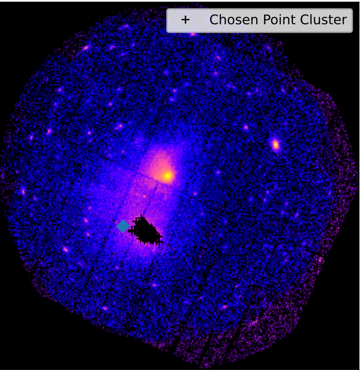
SDSSXCS-71 - Combined 0.5-2.0keV ratemap
