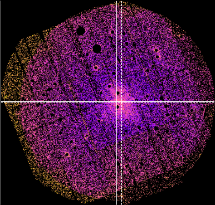
SDSSXCS-7405 - Combined 0.5-2.0keV ratemap
