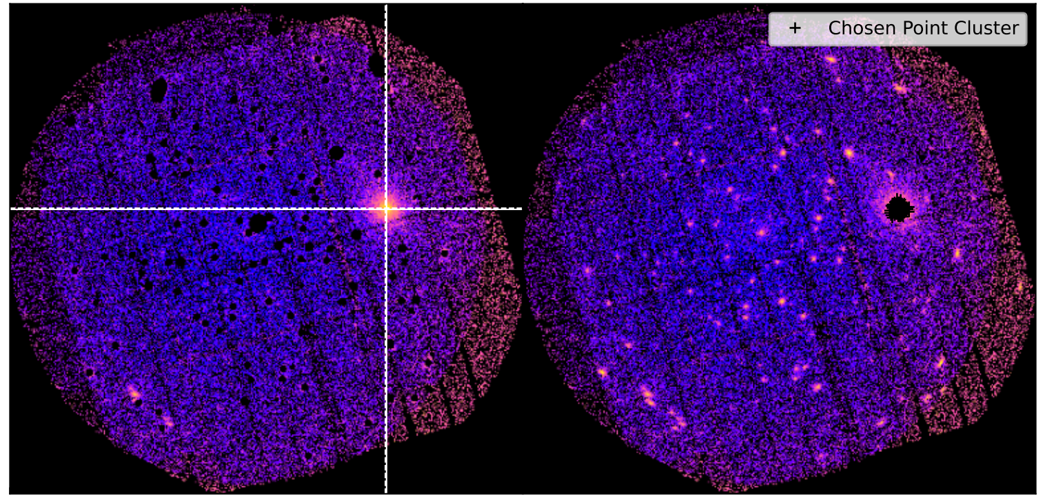
SDSSXCS-7432 - Combined 0.5-2.0keV ratemap SDSSXCS-7432 - Combined 0.5-2.0keV ratemap
