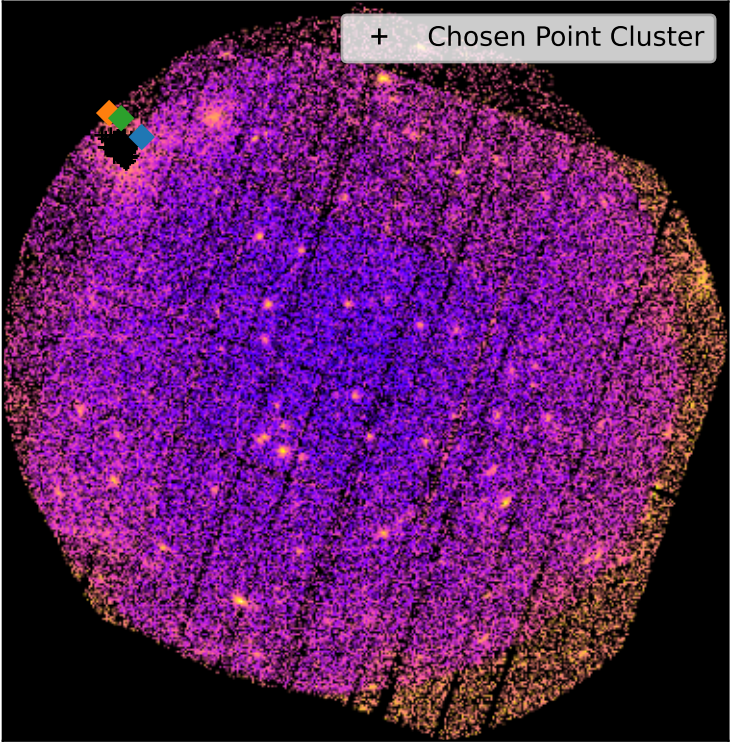
SDSSXCS-765 - Combined 0.5-2.0keV ratemapSDSSXCS-765 - Combined 0.5-2.0keV ratemap
