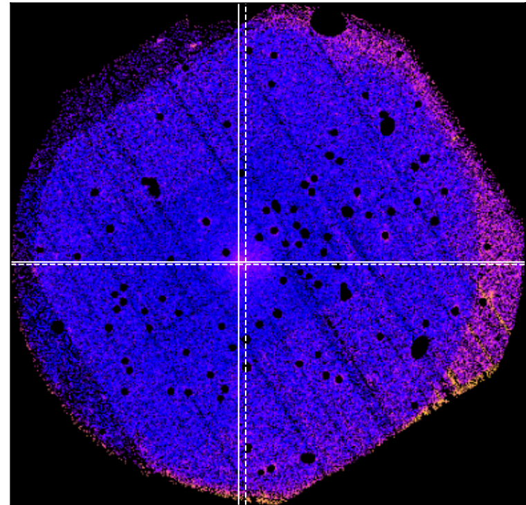
SDSSXCS-9313 - Combined 0.5-2.0keV ratemap
