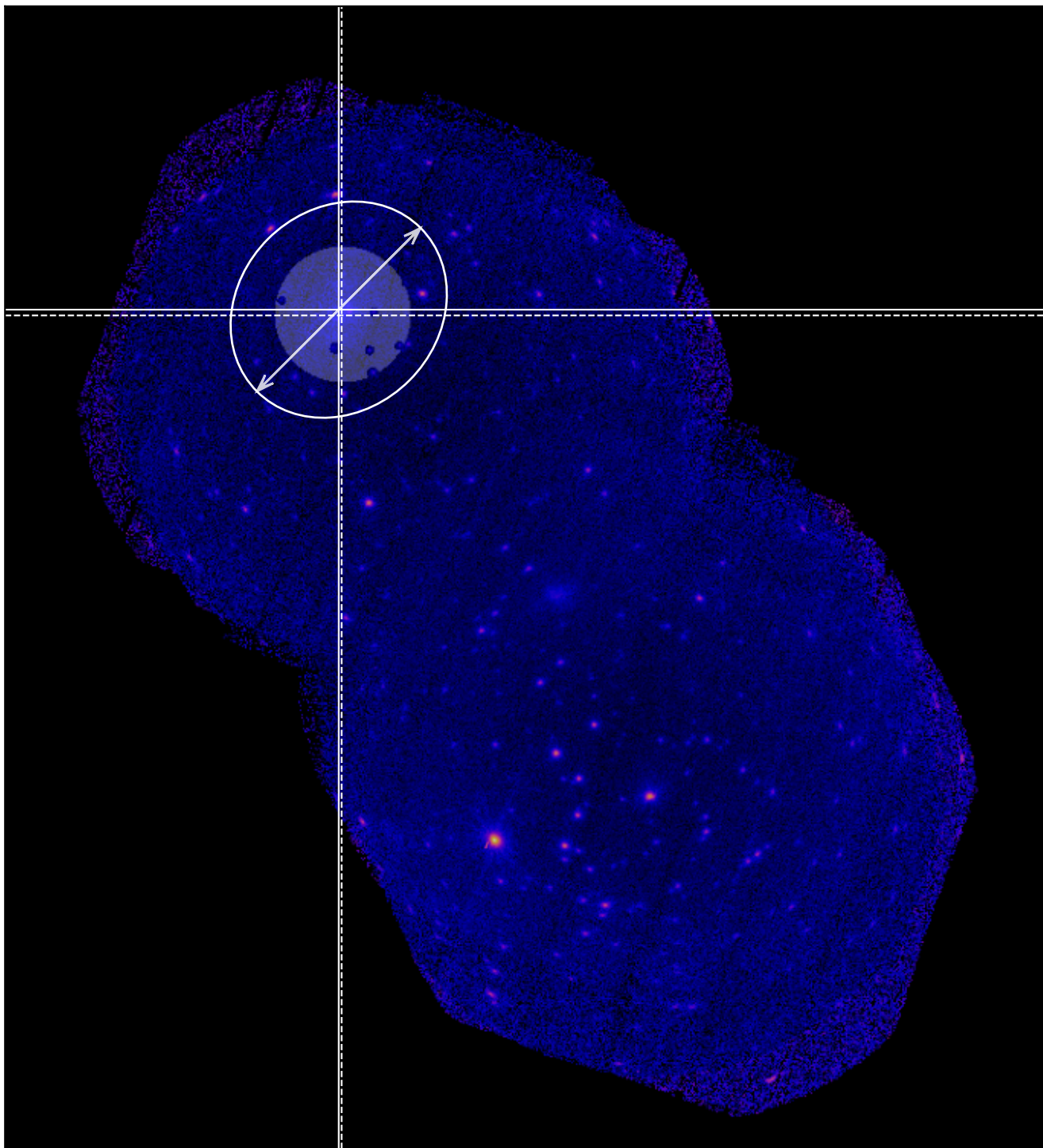
SDSSXCS-10223 - Combined 0.5-2.0keV ratemap
