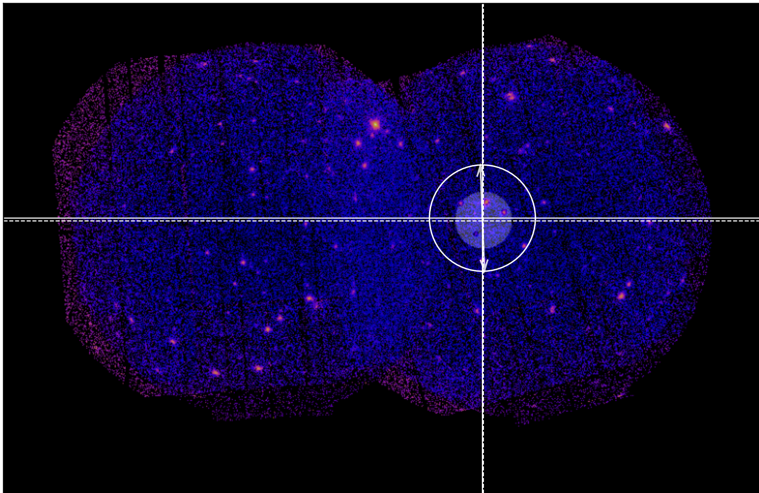
SDSSXCS-30950 - Combined 0.5-2.0keV ratemap
