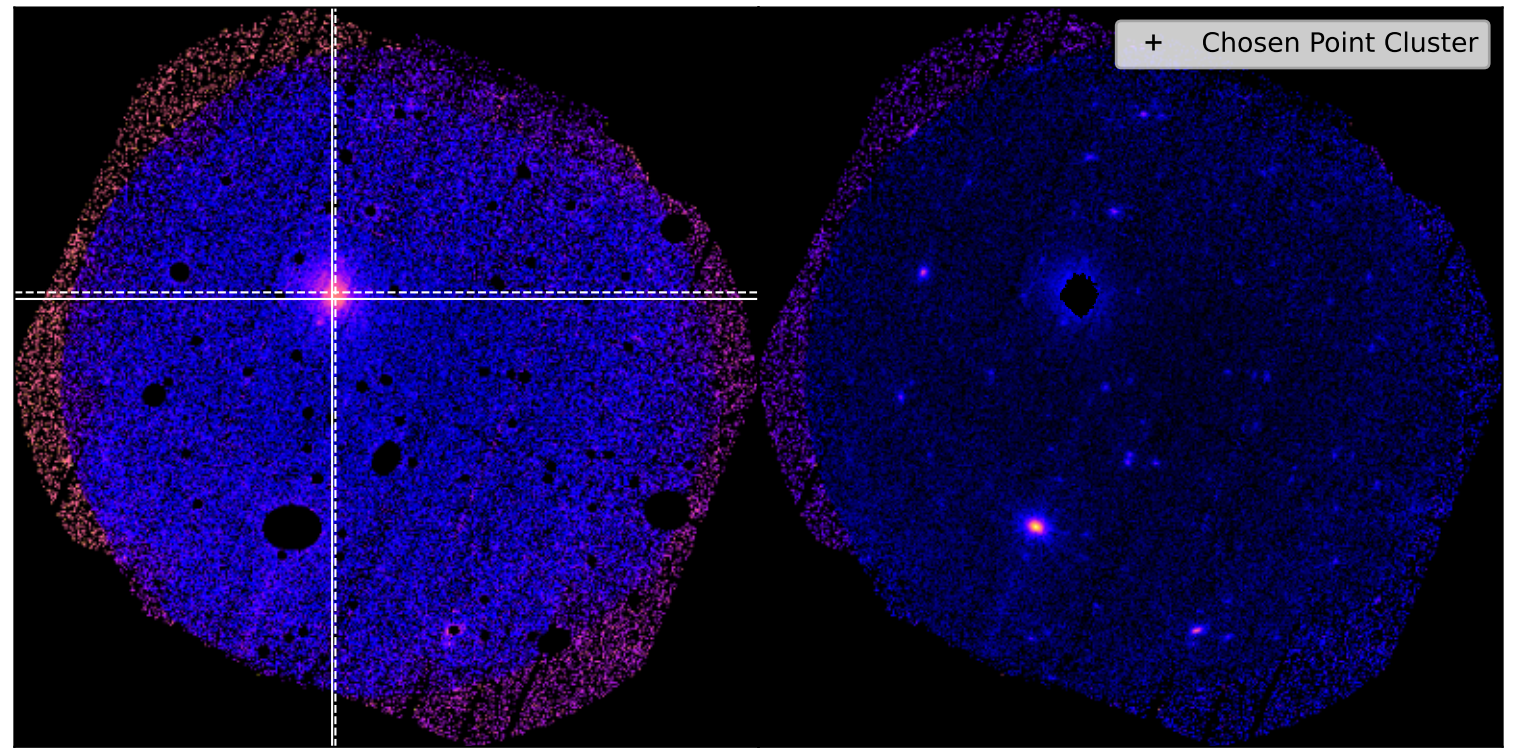
SDSSXCS-1018 - Combined 0.5-2.0keV ratemap
