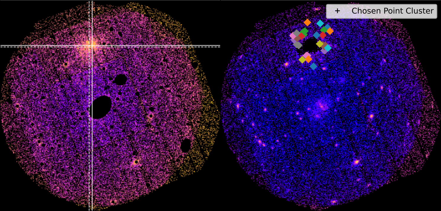
SDSSXCS-10401 - Combined 0.5-2.0keV ratemapSDSSXCS-10401 - Combined 0.5-2.0keV ratemap
