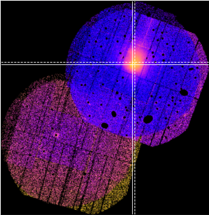
SDSSXCS-110 - Combined 0.5-2.0keV ratemapSDSSXCS-110 - Combined 0.5-2.0keV ratemap
