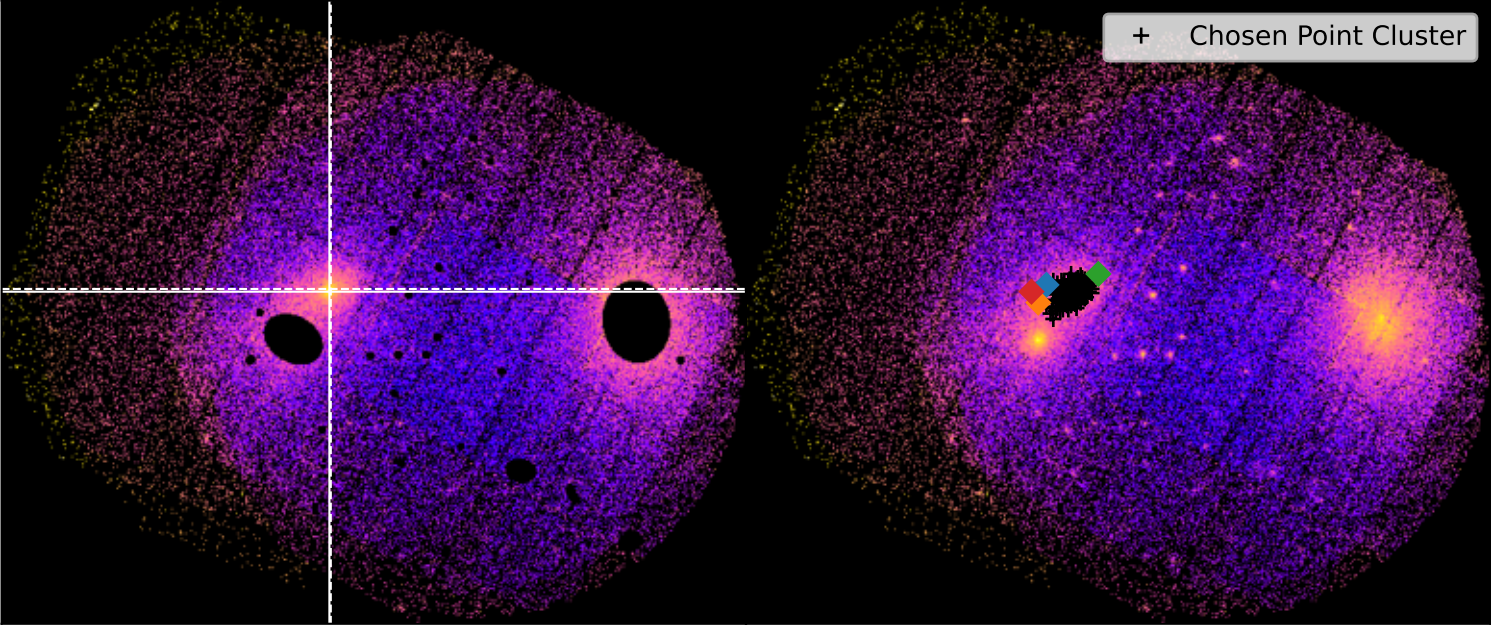
SDSSXCS-11154 - Combined 0.5-2.0keV ratemapSDSSXCS-11154 - Combined 0.5-2.0keV ratemap
