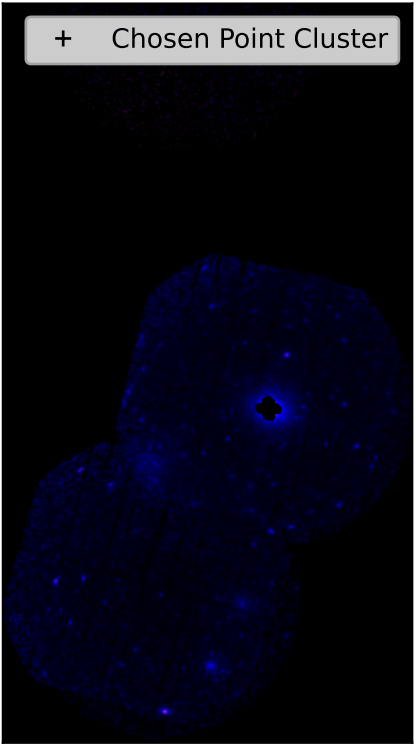
SDSSXCS-1137 - Combined 0.5-2.0keV ratemap
