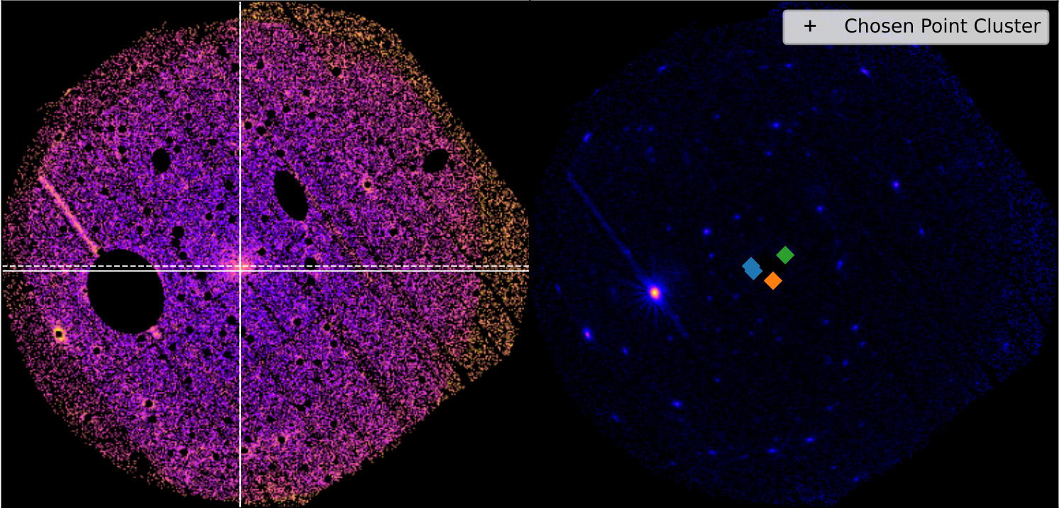
SDSSXCS-11613 - Combined 0.5-2.0keV ratemapSDSSXCS-11613 - Combined 0.5-2.0keV ratemap
