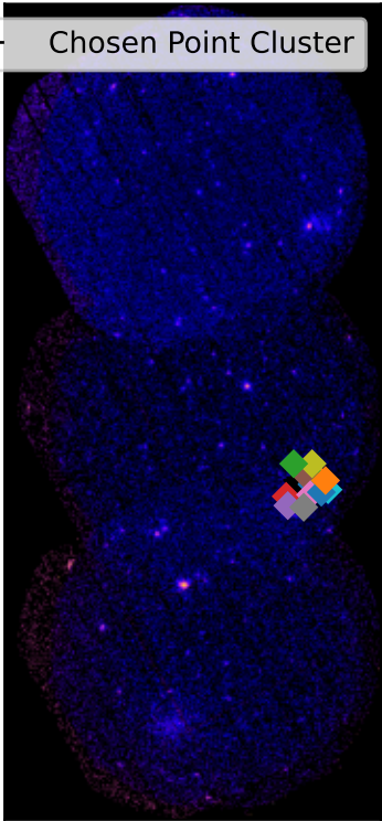
SDSSXCS-1174 - Combined 0.5-2.0keV ratemap
